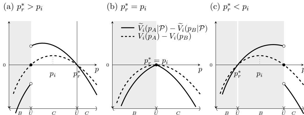
Figure 1: \tilde{V}_i(p_A|\mathcal{P}) - \tilde{V}_i(p_B|\mathcal{P}) given \mathcal{P} = \{p, p_r^*\} B_i(p) = 2\sqrt{p} , C_i(p) = \frac{p^2}{2} , \delta_i = \frac{2}{3}
